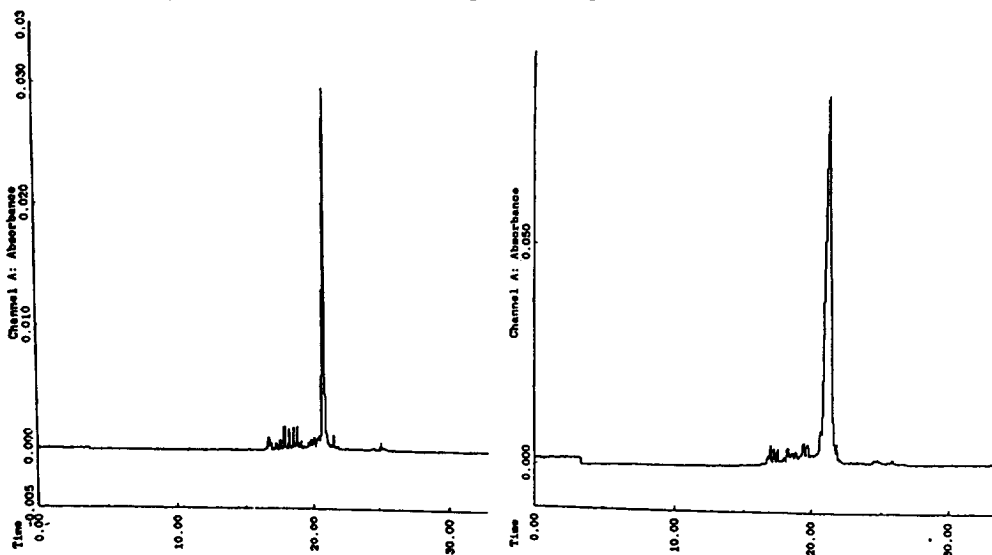
Figure 1: Microgel capillary electrophoretic traces of crude labeled oligonucleotides synthesized using biotin phosphoramidite ( 1a ) and fluorescein phosphoramidite ( 1c ). Panel A: biotinylated oligonucleotide 5'- B-GTA ATG CGA GCG CCA GT-3', where B = biotin. Panel B: fluoresceinated oligonucleotide 5'-F-TGG TCC GCT AAG ACA TTA GT-3', where F = fluorescein.
